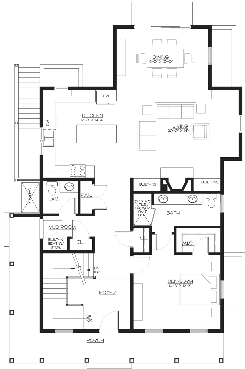
FIRST FLOOR | 1,396 SF
